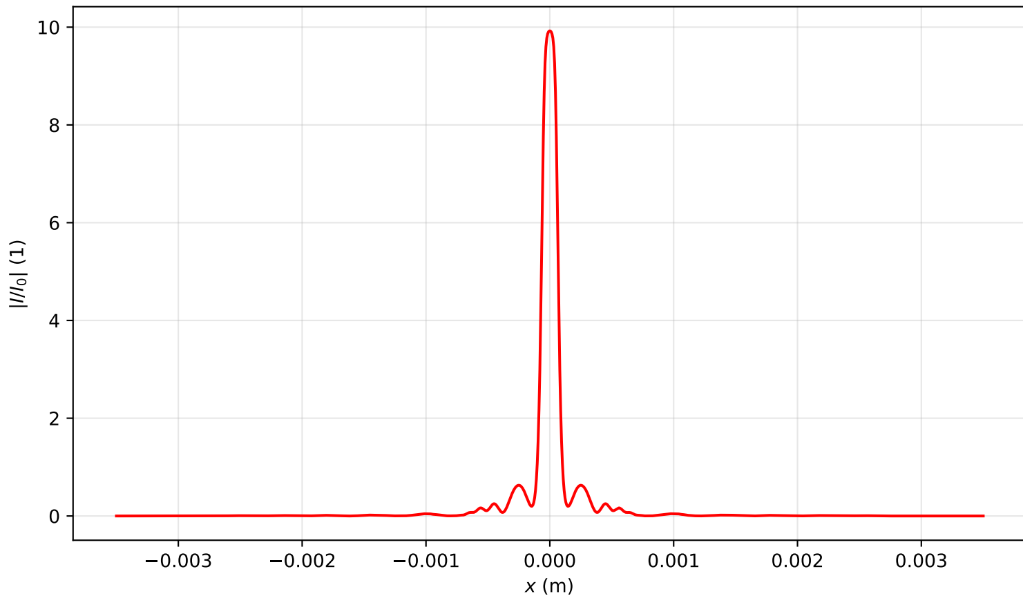
Intensity profile I(x, y = 0, z = 0.318)/I_0 , P_{in}=7.0P_{cr} , artificial time
